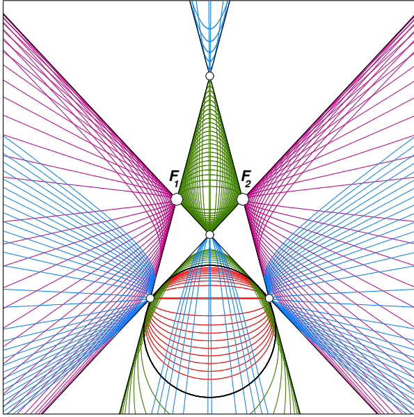
Figure 3: Dual pencil of conics with four common tangents.
