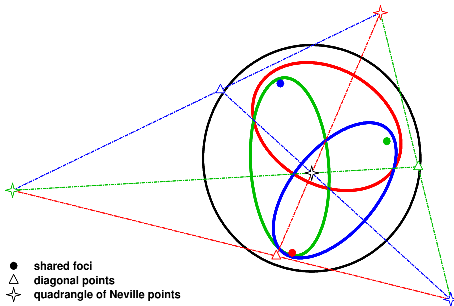
Figure 1: Three focus-sharing conics in Cayley-Klein geometries.
