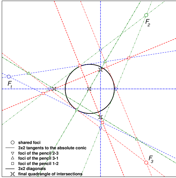
Figure 8: The quadrangle of diagonals of the set of the three pairs of foci.
