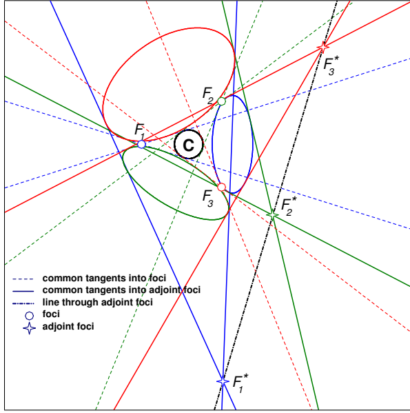
Figure 6: Three focus-sharing conics with their collinear adjoint foci.
