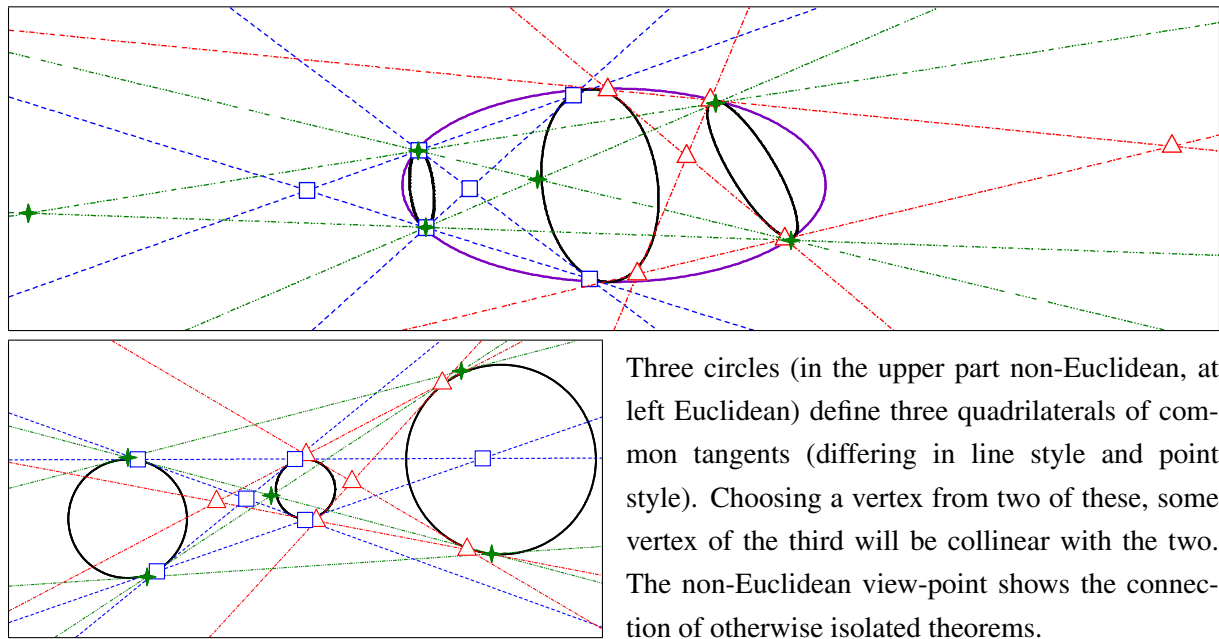
Figure 10: Collinearity between quadrilaterals of common tangents.
