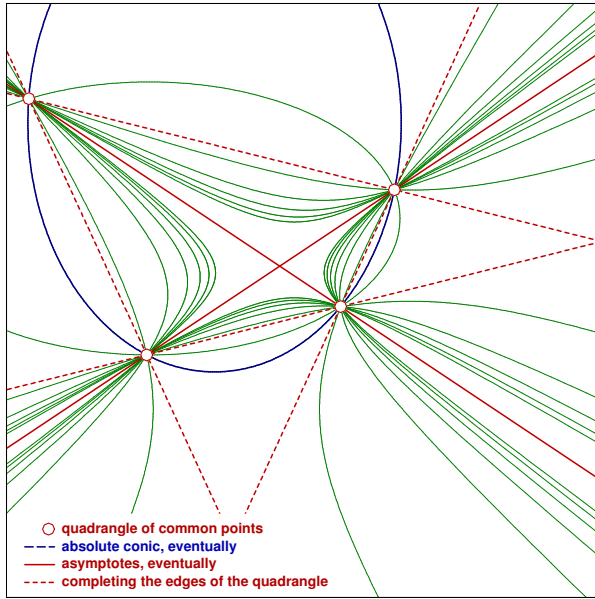
Figure 2: Pencil of conics through four common points.
