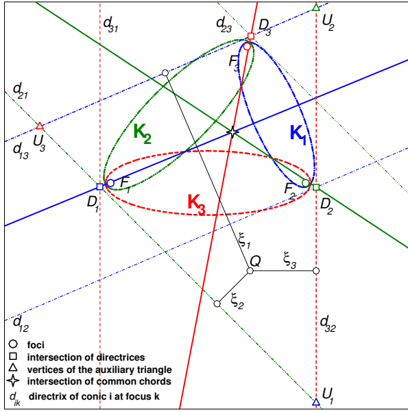
Figure 7: Three focus-sharing ellipses on the Euclidean plane.
